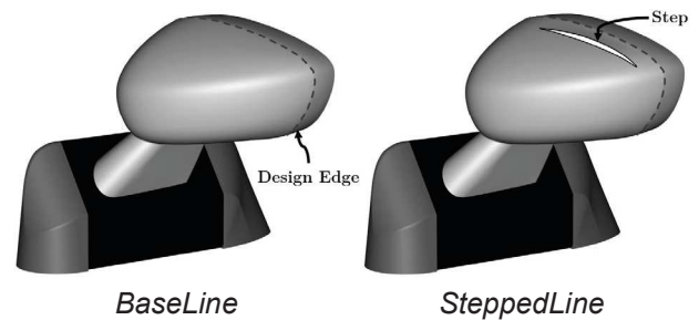
Figure 1: Side-view mirrors designs.
