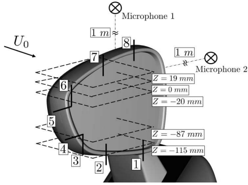
Figure 2: HWA profiles (1 to 8) and TR-PIV planes (noted by their Z-coordinates) recordings locations.
