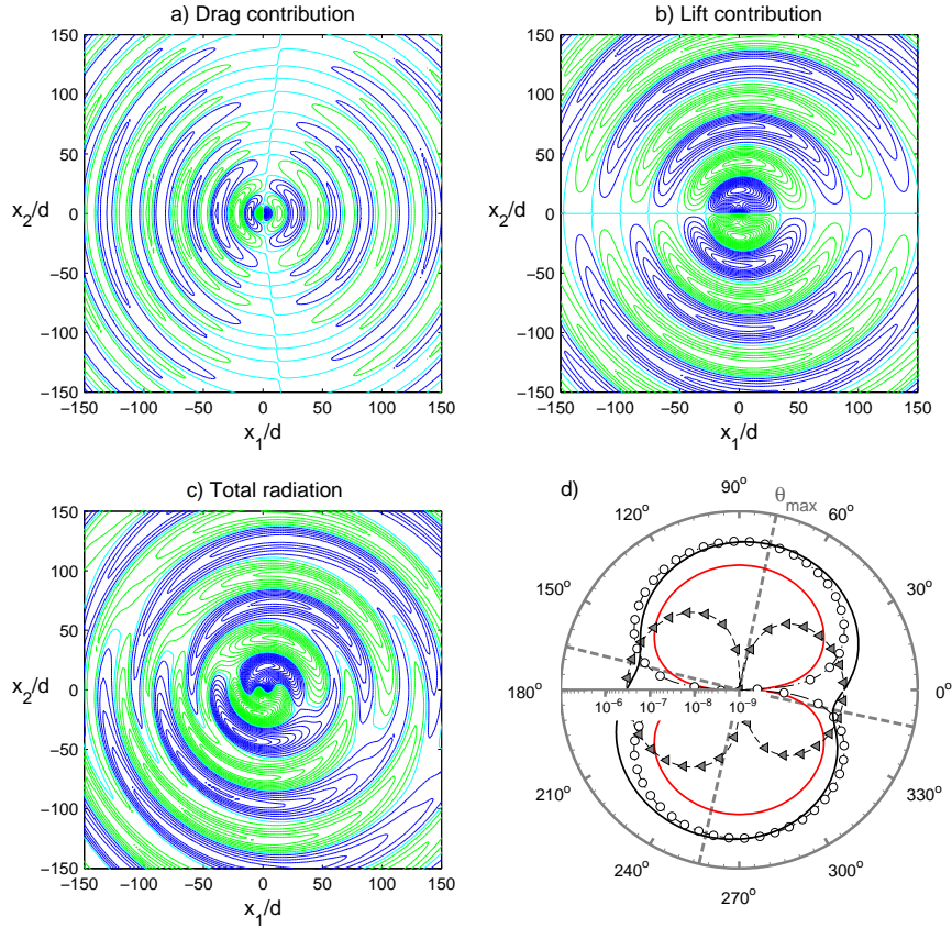
Figure 10: (Color online) Acoustic field for \alpha = 60^\circ and M = 0.1 . Drag (a), lift (b) and total (c) contributions to the pressure field; levels from \pm 0.0004 to \pm 0.02 by step of \pm 0.0006 , blue line: p_a > 0 , green line: p_a < 0 , cyan line: p_a = 0 . Directivity diagram at r/d = 250 (d), triangles: drag contribution, circles: lift contribution, full black line: total noise, red line: total aeolian tone.
