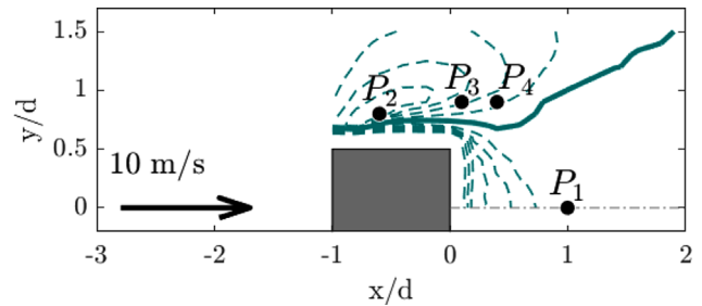
Fig. A.1. Mean flow over a rectangular cylinder of AR = 1 (square cylinder) Re = 6,700 . Isocontours of velocity norm from 0.4 U_\infty to 1.6 U_\infty by step of 0.1 U_\infty . The full, thick line is where U = U_\infty . The labeled bullets ( \bullet ) are the position of the probes in the spanwise study.
