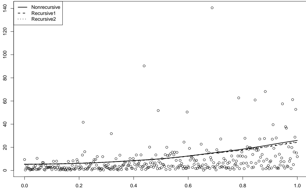
Figure 1: Qualitative comparison between three kernel relative regression estimators; non-recursive correspond to the estimator (5) using the proposed plug-in bandwidth selection (17), Recursive 1 correspond to the estimator (4) using the proposed plug-in bandwidth selection (14) and the stepsize (\gamma_n) = (n^{-1}) , Recursive 2 correspond to the estimator (4) using the proposed plug-in bandwidth selection (14) and the stepsize (\gamma_n) = (h_n / [\sum_{k=1}^n h_k]) using model 1; \mu(X) = 0.5 + 2x , X \sim \mathcal{U}(0, 1) and \varepsilon \sim \mathcal{N}(0, 1) .
