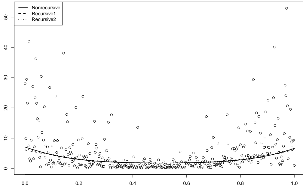
Figure 2: Qualitative comparison between three kernel relative regression estimators; non-recursive correspond to the estimator (5) using the proposed plug-in bandwidth selection (17), Recursive 1 correspond to the estimator (4) using the proposed plug-in bandwidth selection (14) and the stepsize (\gamma_n) = (n^{-1}) , Recursive 2 correspond to the estimator (4) using the proposed plug-in bandwidth selection (14) and the stepsize (\gamma_n) = (h_n / [\sum_{k=1}^n h_k]) using model 2; \mu(X) = \log(0.5 + 40(x - 0.5)^2) , X \sim \mathcal{U}(0, 1) and \varepsilon \sim \mathcal{N}(0, 1) .
