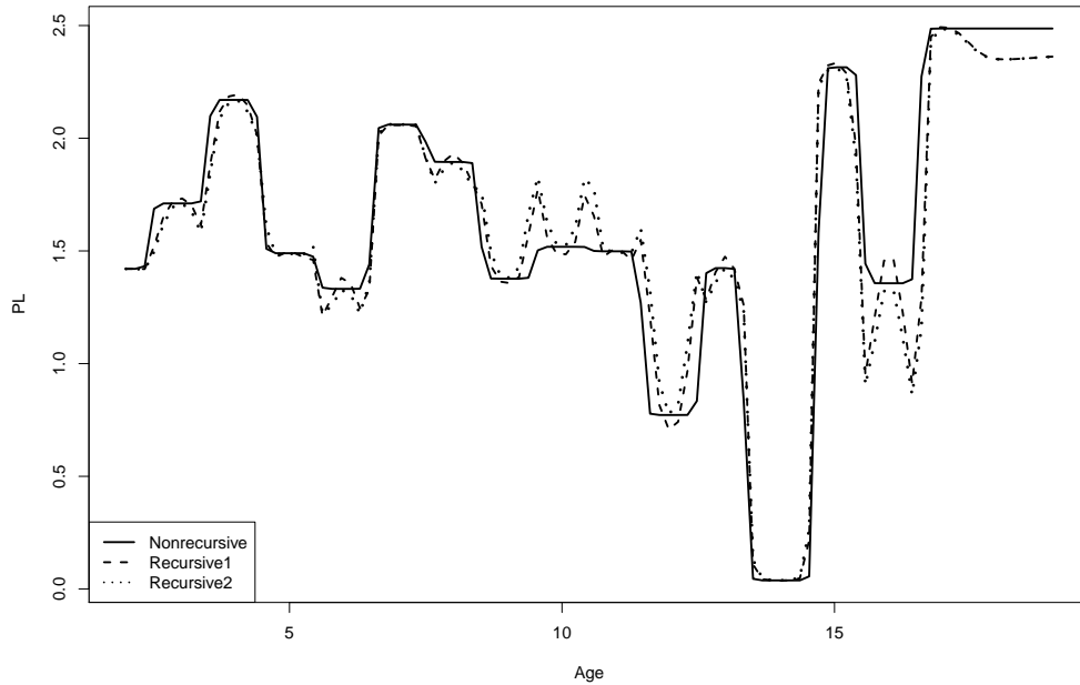
Figure 3: The Plasmodium falciparum Parasite Load density with automatically bandwidth selection using the Non-recursive correspond to the estimator (5) using the proposed plug-in bandwidth selection (17), Recursive 1 correspond to the estimator (4) using the proposed plug-in bandwidth selection (14) and the stepsize (\gamma_n) = (n^{-1}) , Recursive 2 correspond to the estimator (4) using the proposed plug-in bandwidth selection (14) and the stepsize (\gamma_n) = (h_n / [\sum_{k=1}^n h_k]) .
